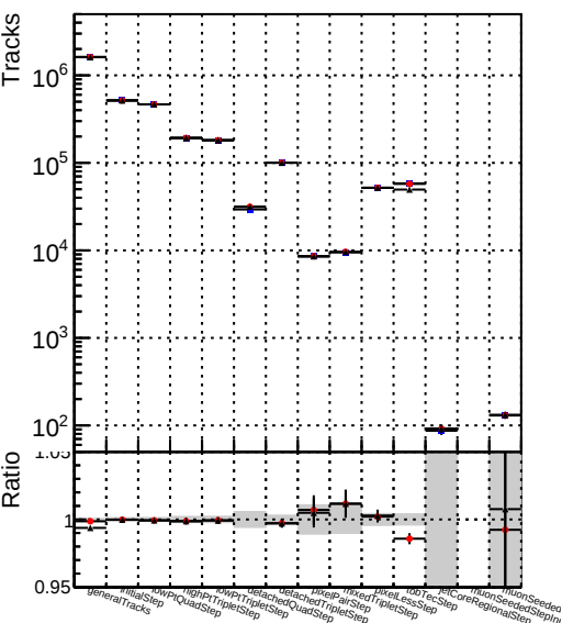
Number Legend DQM_V0001_R000000001_Global_mkFitOLD_RECO DQM_V0001_R000000001_Global_mkFit100_RECO DQM_V0001_R000000001_Global_mkFit100tobtec_RECO
