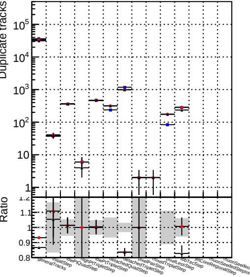
DQM_V0001_R0000000001_Global_mkFitOLD_RECO DQM_V0001_R0000000001_Global_mkFit100_RECO Number DQM_V0001_R0000000001_Global_mkFit100tobtec_RECO
