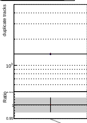
N of associated (recoToSim) loopier tracks vs. \chi^2
