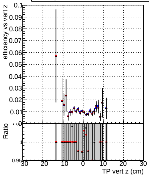
Efficiency vs TP vert z —●— DQM_V0001_R0000000001_Global_mkFitOLD_RECO —●— DQM_V0001_R0000000001_Global_mkFit100_RECO —●— DQM_V0001_R0000000001_Global_mkFit100tobtec_RECO
