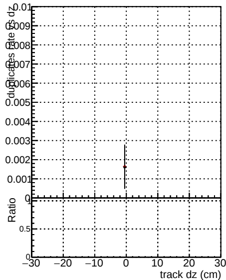
DOM V0001 RECO DOM V0001 RECO Global mkFitOLD RECO Global mkFit100 RECO
