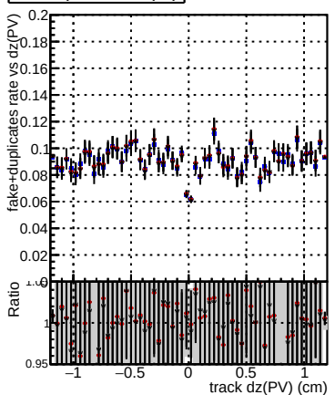
fake+duplicates vs dz(PV) (Zoomed)
