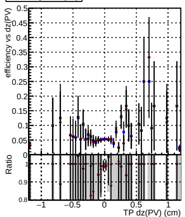
Efficiency vs Dz(PV) (Zoomed)
