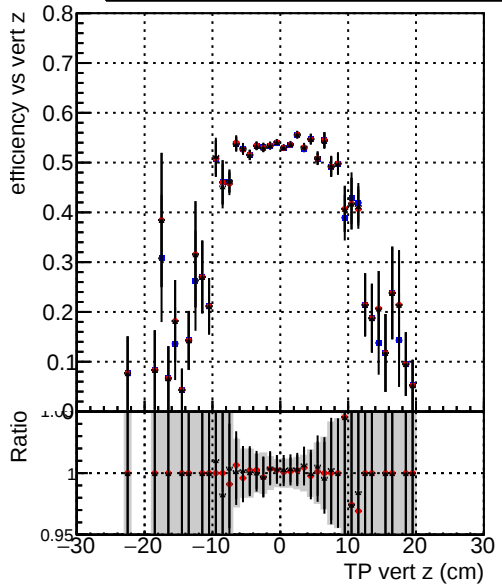
Efficiency vs vert z —●— DQM_V0001_R000000001_Global_mkFitOLD_RECO —●— DQM_V0001_R000000001_Global_mkFit100_RECO —●— DQM_V0001_R000000001_Global_mkFit100tobtec_RECO
