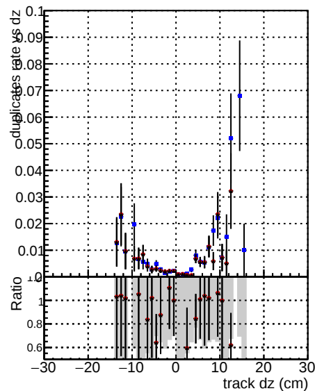
DOM V0001 DOM V0001 RECO Global mkFitOLD RECO DOM V0001 DOM V0001 RECO Global mkFit100 RECO
