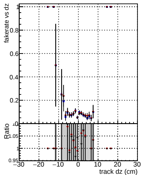
Fake rate vs dz Global fit OLD RECO Global fit OLD RECO Global fit OLD RECO Global fit OLD RECO Global fit OLD RECO Global fit OLD RECO Global fit OLD RECO Global fit OLD RECO Global fit OLD RECO
