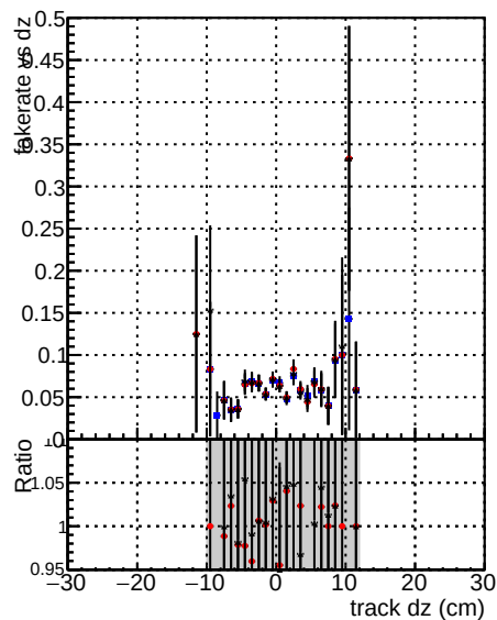
DOM V0001 R0000000001 Global mkFitOLD RECO Fake rate vs d Blue line with dots Red line with dots Black line with dots Black line with dots Duplicates Rate vs Dxy Blue line with dots Red line with dots Black line with dots Black line with dots Pileup rate vs dxy Blue line with dots Red line with dots Black line with dots Black line with dots
