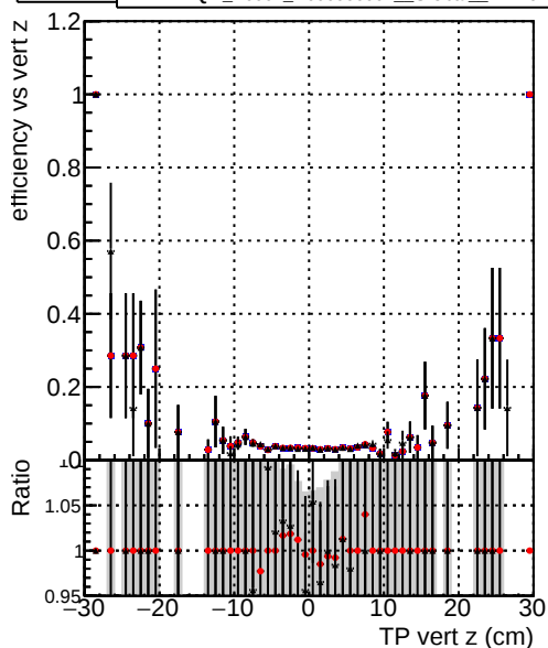
Efficiency vs vert z —●— DQM_V0001_R0000000001_Global_mkFitOLD_RECO —●— DQM_V0001_R0000000001_Global_mkFit100_RECO —●— DQM_V0001_R0000000001_Global_mkFit100tobtec_RECO
