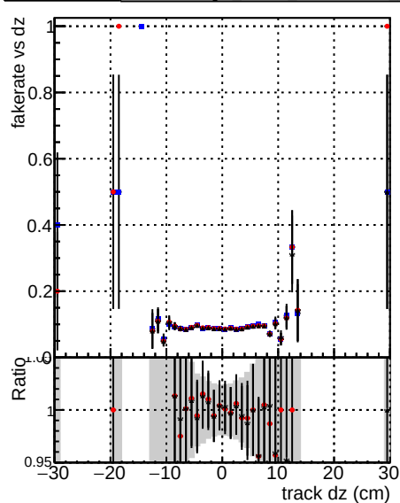
DOM V0001 R0000000001 Global mkFitOLD RECO DOM V0001 R0000000001 Global mkFit100 RECO DOM V0001 R0000000001 Global mkFit100robtec RECO
