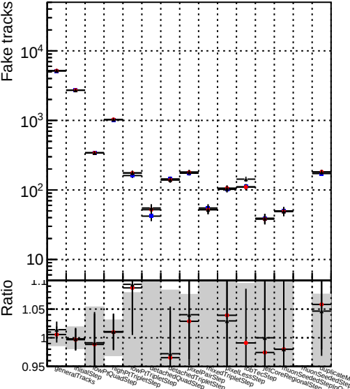
Number Label Model Fit Reco 1 DQM_V0001_R0000000001 Global mkFitOLD RECO 2 DQM_V0001_R0000000001 Global mkFit100 RECO 3 DQM_V0001_R0000000001 Global mkFit100tobtcc RECO
