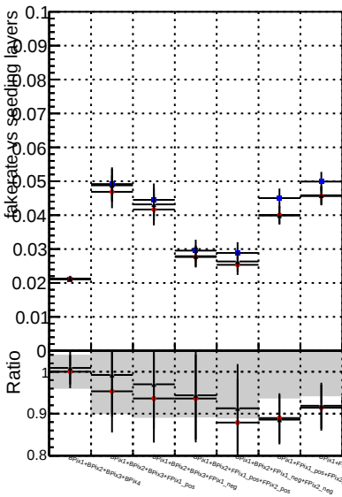
Fake rate vs. Legend Global mkFitOLD RECO DOM V0001 R0000000001 DOM V0001 R0000000001 DOM V0001 R0000000001
