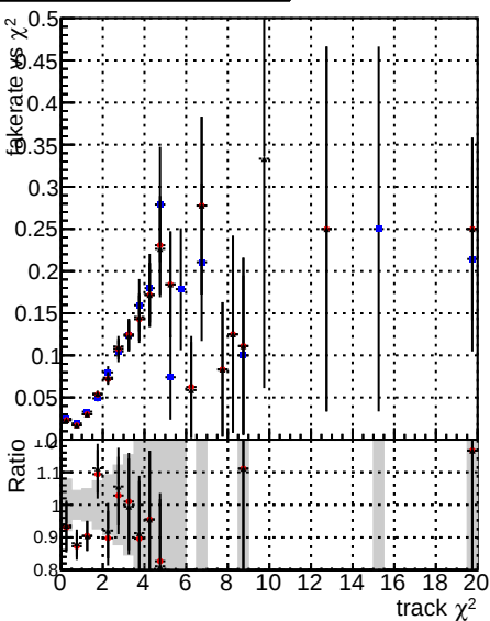
Fake rate vs. Legend Global mkFitOLD RECO DOM V0001 R0000000001 DOM V0001 R0000000001 DOM V0001 R0000000001
