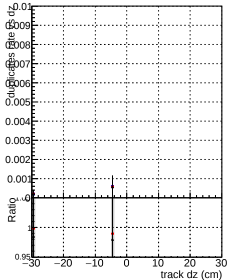
Legend for all plots: DOM V0001 RECO (black squares) DOM V0001 RECO (red circles) Global mkFit100 RECO (blue triangles) Global mkFit100 RECO (black squares) Global mkFit100 RECO (red circles) Global mkFit100 RECO (blue triangles)
