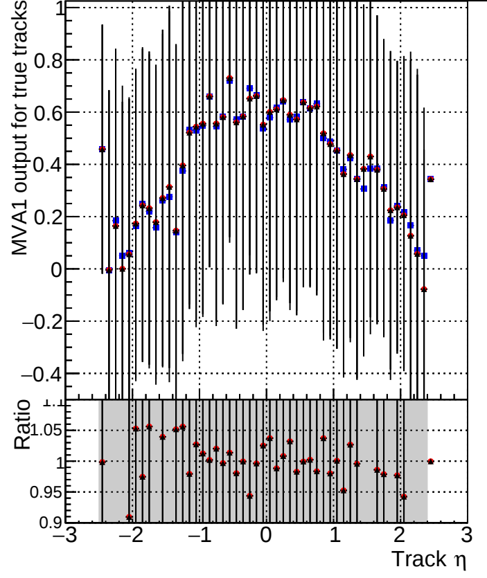
MVA1 of associated tracks (recoToSim) vs. track \eta ■ DQM_V0001_R000000001_Global_mkFitOLD_RECO ● DQM_V0001_R000000001_Global_mkFit100_RECO ▲ DQM_V0001_R000000001_Global_mkFit100tobtec_RECO
