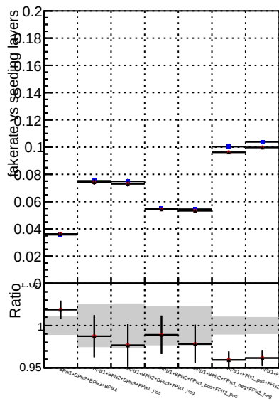
Fake rate vs. DOM V0001 R0000000001 Global mkFitOLD RECO DOM V0001 R0000000001 Global mkFit100 RECO DOM V0001 R0000000001 Global mkFit100robtec RECO
