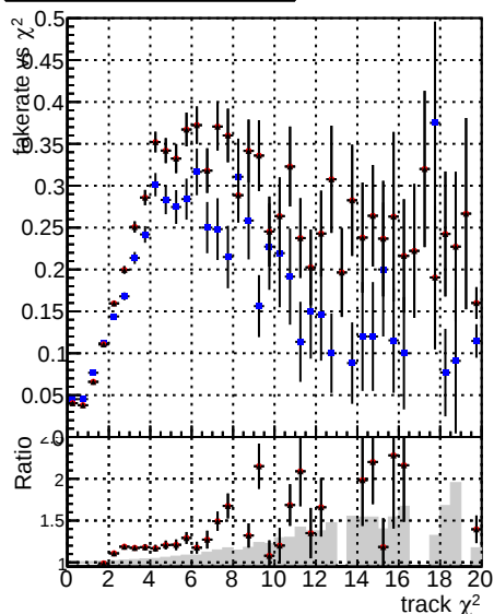
Fake rate vs. DOM V0001 R0000000001 Global mkFitOLD RECO DOM V0001 R0000000001 Global mkFit100 RECO DOM V0001 R0000000001 Global mkFit100robtec RECO
