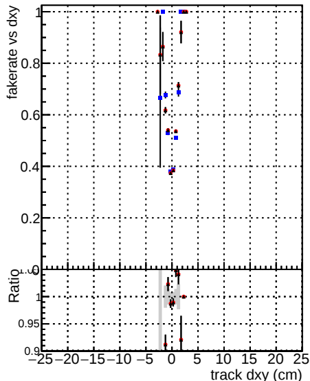
DOM V0001 DOM V0001 RECO Global mKFitOLD RECO DOM V0001 DOM V0001 RECO Global mKFitOLD RECO DOM V0001 DOM V0001 RECO Global mKFitOLD RECO
