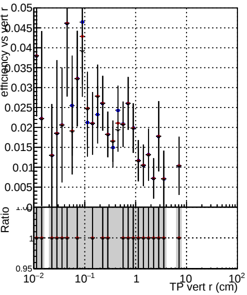
Efficiency vs vertpos —●— DQM_V0001_R0000000001_Global_mkFitOLD_RECO —●— DQM_V0001_R0000000001_Global_mkFit100_RECO —●— DQM_V0001_R0000000001_Global_mkFit100tobtec_RECO
