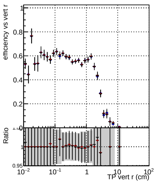
Efficiency vs TP vert r (cm) —●— DQM_V0001_R000000001_Global_mkFitOLD_RECO —●— DQM_V0001_R000000001_Global_mkFit100_RECO —●— DQM_V0001_R000000001_Global_mkFit100tobtec_RECO
