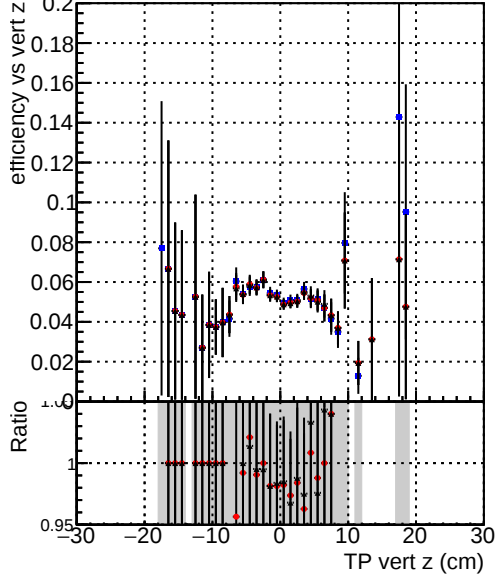
Efficiency vs. TP vert z —●— DQM_V0001_R000000001_Global_mkFitOLD_RECO —●— DQM_V0001_R000000001_Global_mkFit100_RECO —●— DQM_V0001_R000000001_Global_mkFit100tobtec_RECO
