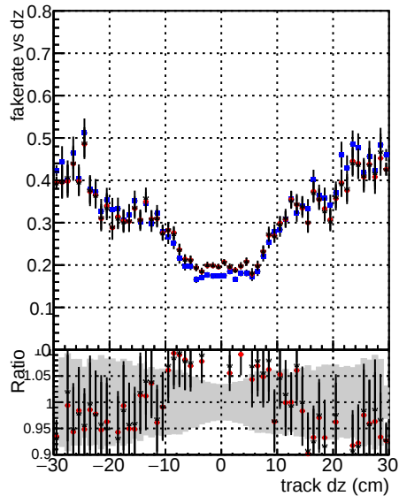
DOM V0001 DOM V0001 RECO Global fit OLD RECO DOM V0001 DOM V0001 RECO Global fit OLD RECO DOM V0001 DOM V0001 RECO Global fit OLD RECO
