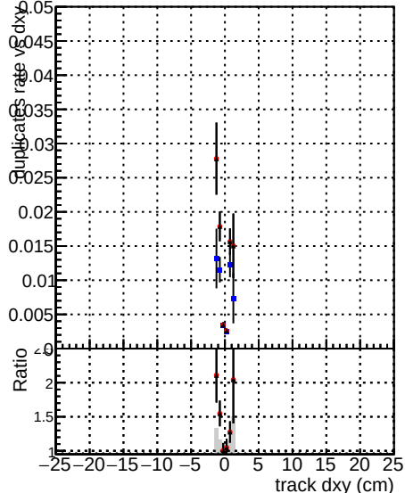
DOM V0001 DOM V0001 RECO Global fit Global fit OLD RECO Global fit OLD RECO DOM V0001 DOM V0001 RECO Global fit Global fit OLD RECO Global fit OLD RECO DOM V0001 DOM V0001 RECO Global fit Global fit OLD RECO Global fit OLD RECO
