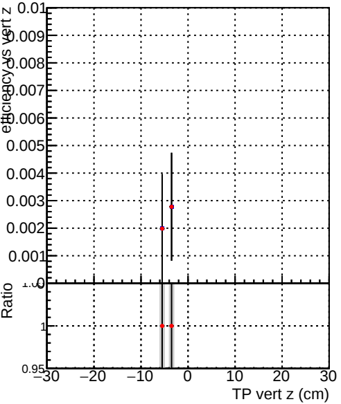
Efficiency vs TP vert z (cm) Legend: DQM_V0001_R0000000001_Global_mkFit100o_RECO DQM_V0001_R0000000001_Global_mkFit100_RECO
