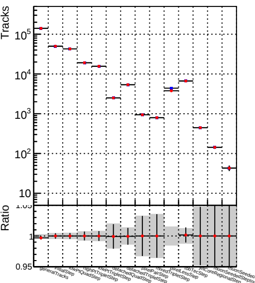
DQM_V0001_R000000001__Global__mkFit100o__RECO
