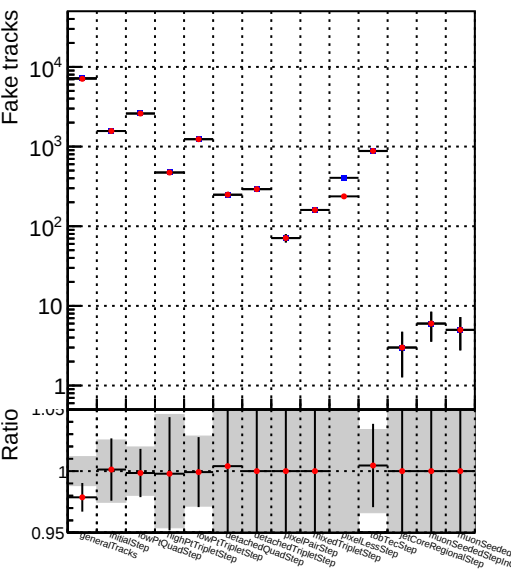
Number —●— DQM_V0001_R000000001_Global_mkFit100_RECO
