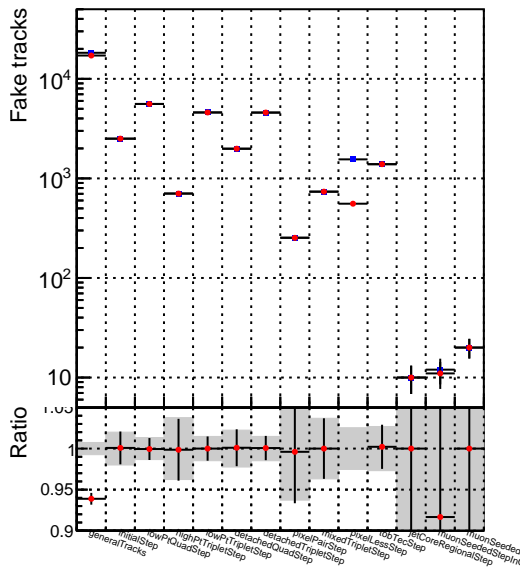
● DQM_V0001_R000000001_Global_mkFit100_RECO
