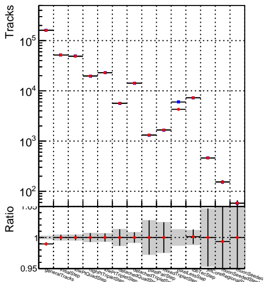
— DQM_V0001_R000000001_Global_mkFit100o_RECO
