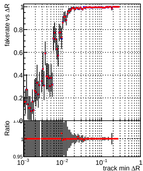
—●— DQM_V0001_R000000001_Global_mkFit100o_RECO —●— DQM_V0001_R000000001_Global_mkFit100_RECO
