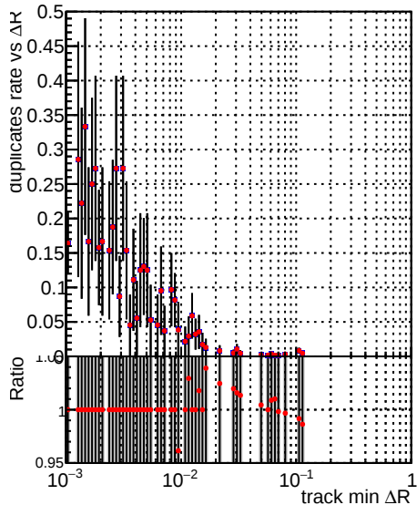
—●— DQM_V0001_R000000001_Global_mkFit100o_RECO —●— DQM_V0001_R000000001_Global_mkFit100_RECO
