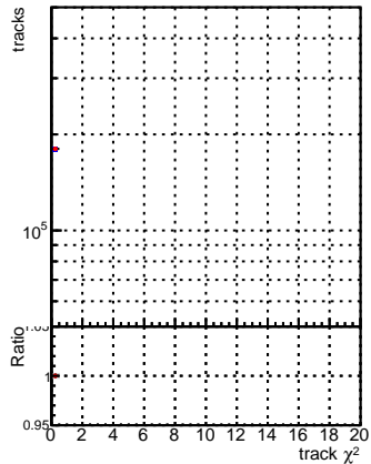
Global_mkFit100o_RECO Global_mkFit100o_RECO
