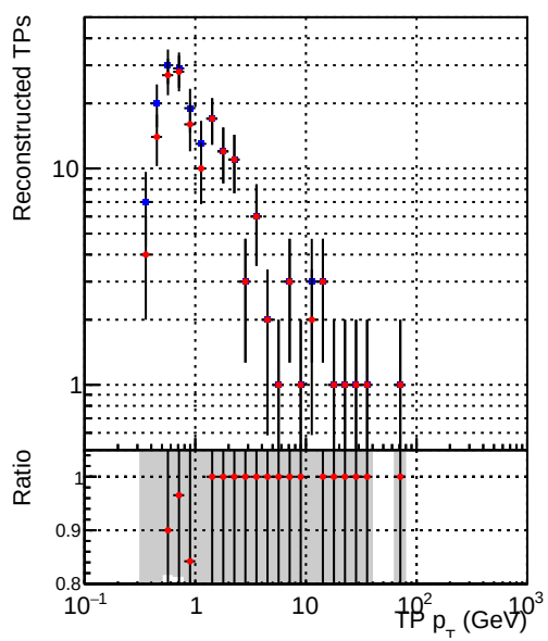
Legend: DQM_V0001_R000000001_Global_mkFit100o_RECO (blue dots), DQM_V0001_R000000001_Global_mkFit100_RECO (red dots)
