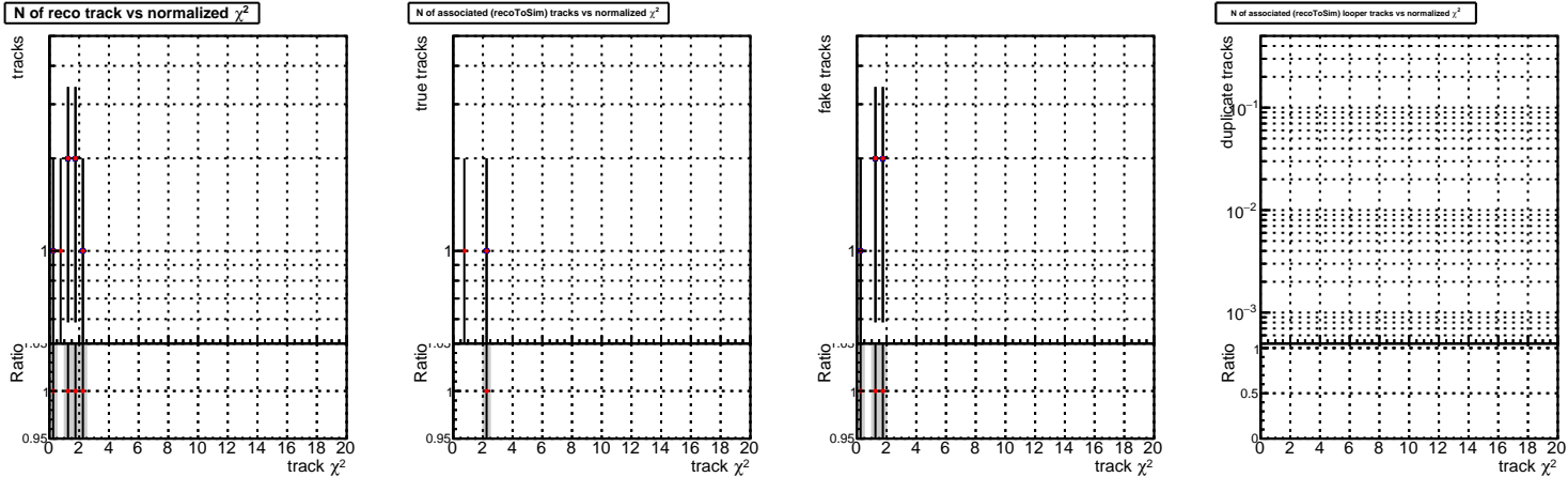
—•— DQM_V0001_R0000000001_Global_mkFit100o_RECO —•— DQM_V0001_R0000000001_Global_mkFit100_RECO
