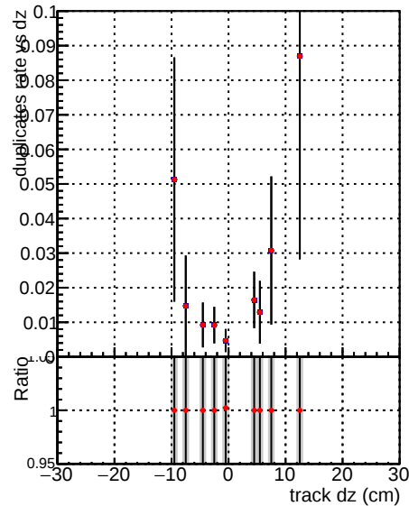
al__mkFit100o__RECO al__mkFit100__RECO
