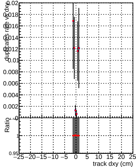
al__mkFit100o__RECO al__mkFit100__RECO
