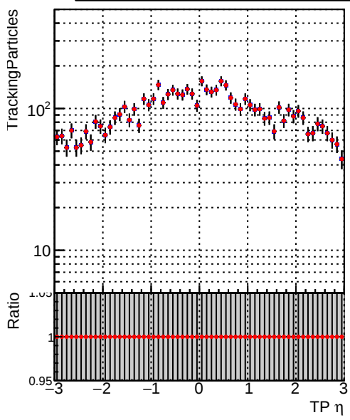
Legend: DQM_V0001_R0000000001_Global_mkFit100o_RECO (blue line), DQM_V0001_R0000000001_Global_mkFit100_RECO (red line)
