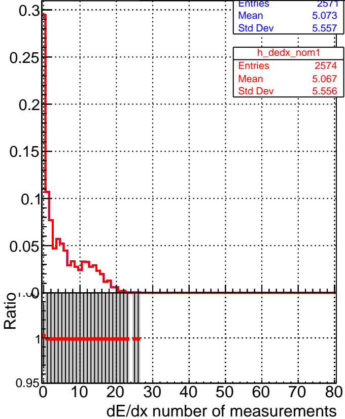
■ DQM_V0001_R000000001_Global_mkFit100o_RECO ● DQM_V0001_R000000001_Global_mkFit100_RECO
