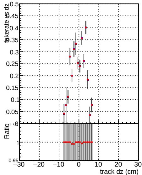
—•— DQM_V0001_R0000000001_Global_mkFit100o_RECO —•— DQM_V0001_R0000000001_Global_mkFit100o_RECO
