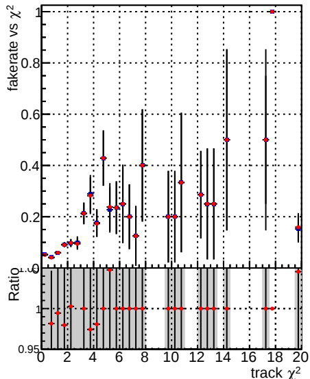
Fake rate vs. —●— DQM V0001_R000000001_Global_mkFit100o_RECO —●— DQM V0001_R000000001_Global_mkFit100_RECO
