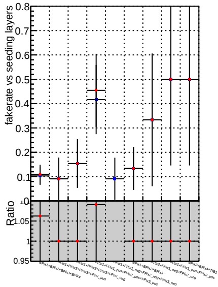
Fake rate vs. —•— DQM V0001_R000000001 Global mkFit100o RECO —•— DQM V0001_R000000001 Global mkFit100 RECO
