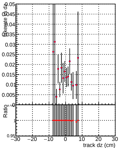
Legend Fake rate vs dz DQM_V0001_R0000000001_Global_mkFit100o_RECO DQM_V0001_R0000000001_Global_mkFit100o_RECO
