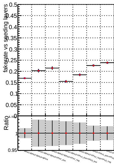
Fake rate vs. —•— DQM_V0001_R0000000001_Global_mkFit100o_RECO —•— DQM_V0001_R0000000001_Global_mkFit100_RECO
