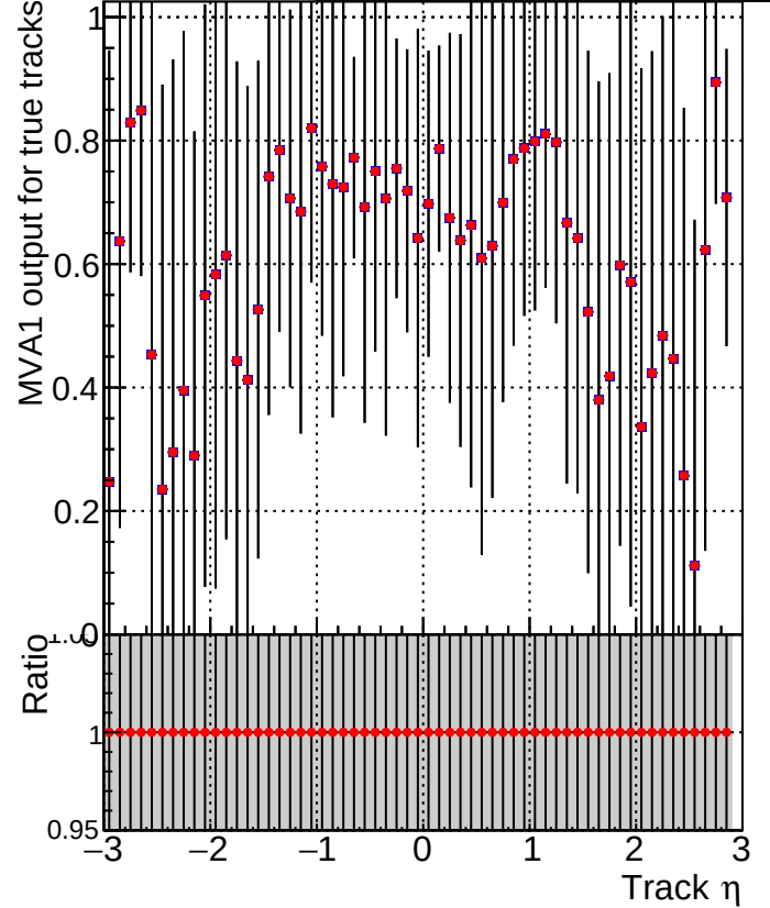
MVA1 of associated tracks (recoToSim) vs. track \eta Legend: ■ DQM_V0001_R000000001_Global_mkFit100o_RECO ● DQM_V0001_R000000001_Global_mkFit100_RECO
