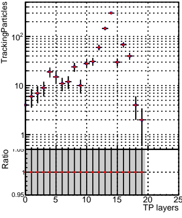
DQM_V0001_R000000001_Global_mkFit100o_RECO
