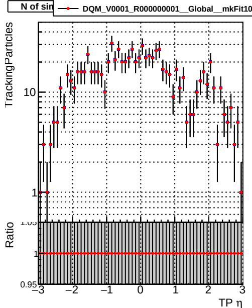
N of simulated tracks vs \eta
