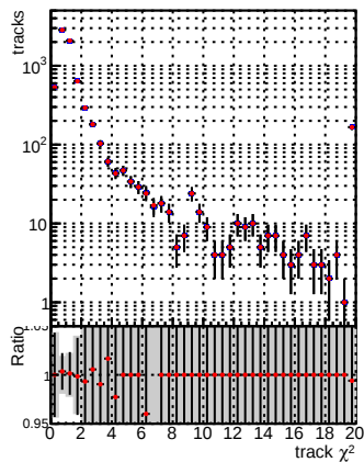
N of reco track vs. —●— DQM_V0001_R0000000001_Global_mkFit100o_RECO —●— DQM_V0001_R0000000001_Global_mkFit100o_RECO
