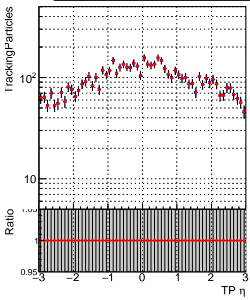
N of simulated tracks vs TP \eta Legend: - DQM_V0001_R000000001_Global_mkFit100o_RECO (blue points) - DQM_V0001_R000000001_Global_mkFit100_RECO (red points)
