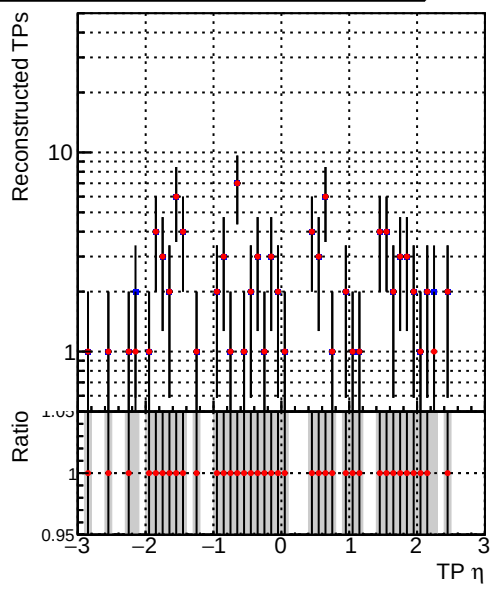
—•— DQM_V0001_R000000001_Global_mkFit100o_RECO —•— DQM_V0001_R000000001_Global_mkFit100_RECO
