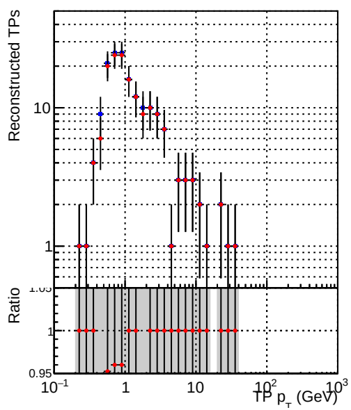
—•— DQM_V0001_R000000001_Global_mkFit100o_RECO —•— DQM_V0001_R000000001_Global_mkFit100_RECO
