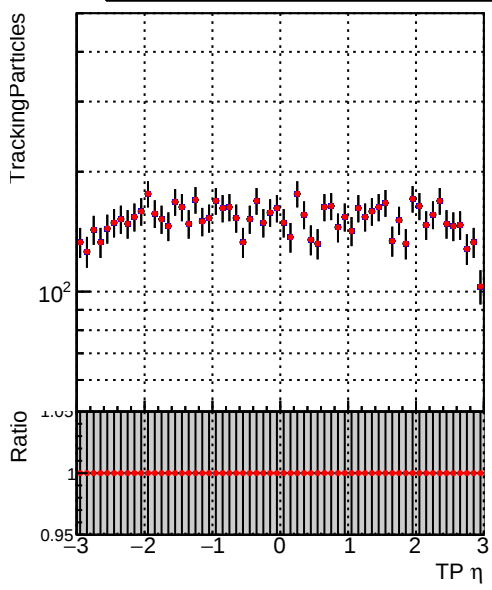
Legend: DQM_V0001_R0000000001_Global_mkFit100o_RECO (blue line), DQM_V0001_R0000000001_Global_mkFit100dt_RECO (red line)
