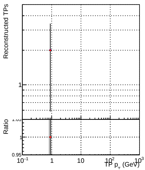
Legend: DQM_V0001_R0000000001_Global_mkFit100o_RECO (blue line), DQM_V0001_R0000000001_Global_mkFit100dt_RECO (red line)
