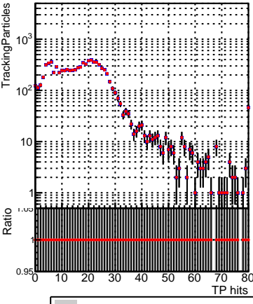
N of sim ■ DQM_V0001_R000000001_Global_mkFit100o_RECO ■ DQM_V0001_R000000001_Global_mkFit100dt_RECO
