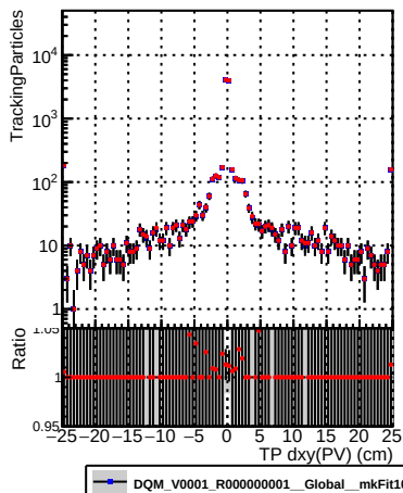
N of sim DQM_V0001_R000000001_Global_mkFit100dt_RECO
