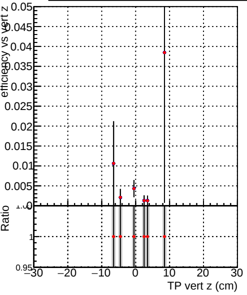
Efficiency vs TP vert z (cm) Legend: DQM_V0001_R000000001_Global_mkFit100o_RECO DQM_V0001_R000000001_Global_mkFit100dt_RECO
