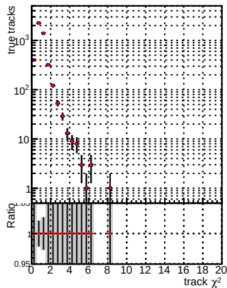
Global mkFit100e RECO Global mkFit100dt RECO
