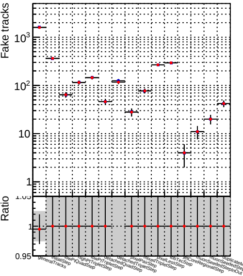
Number —●— DOM V0001 R0000000001 Global mkFit100dt RECO
